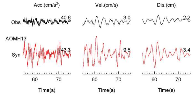
(2) EW Component
