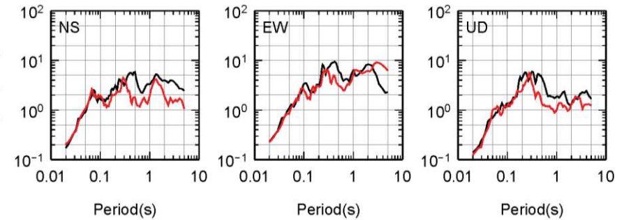
KiK-net IWTH27
