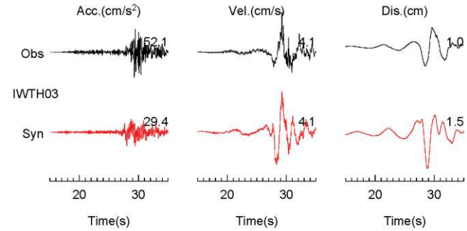
(1) NS Component
