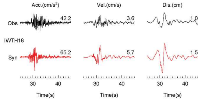
(1) NS Component
