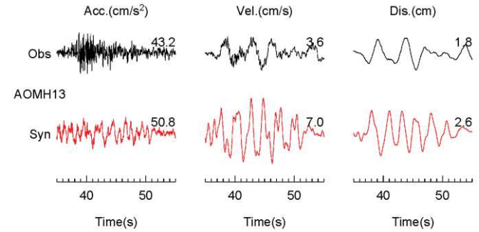
(1) NS Component
