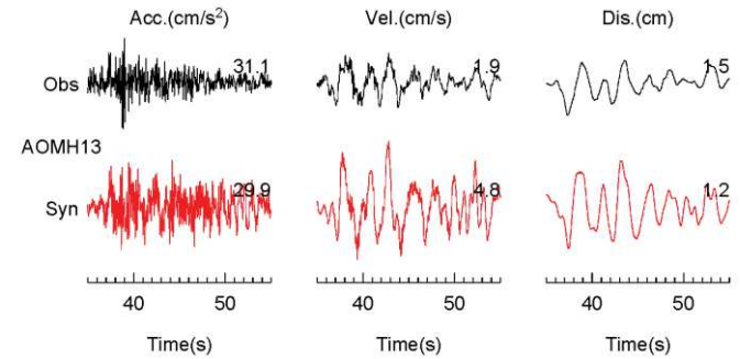
(3) UD Component
