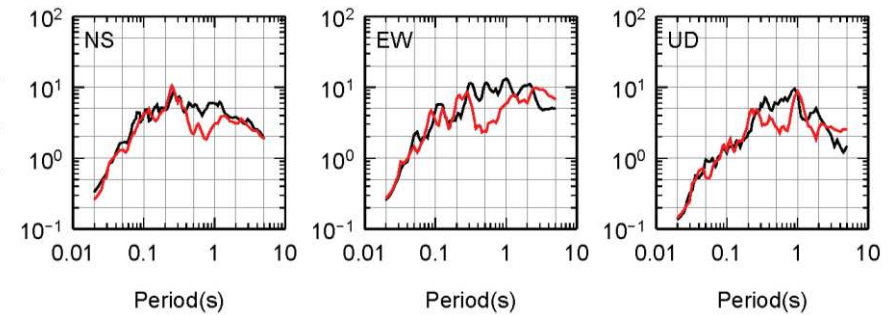
KiK-net IWTH23
