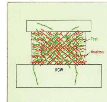
Fig.1.1b Cracks appeared - analysis and test (RCW)
