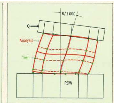
Fig.1.1c Shape of total deformation - analysis and test (RCW)
