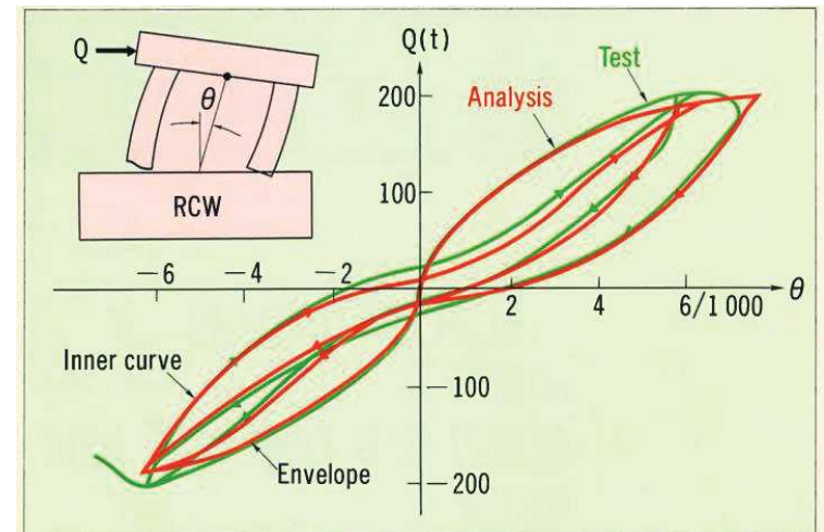
Fig.1.1a Rotational angles of specimen RCW - analysis and test
